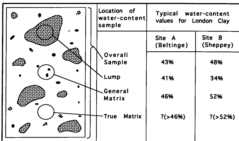
FIGURE 3-18 Mudslide fabric and associated variability in water content (modified from Hutchinson 1988, Figure 9).
