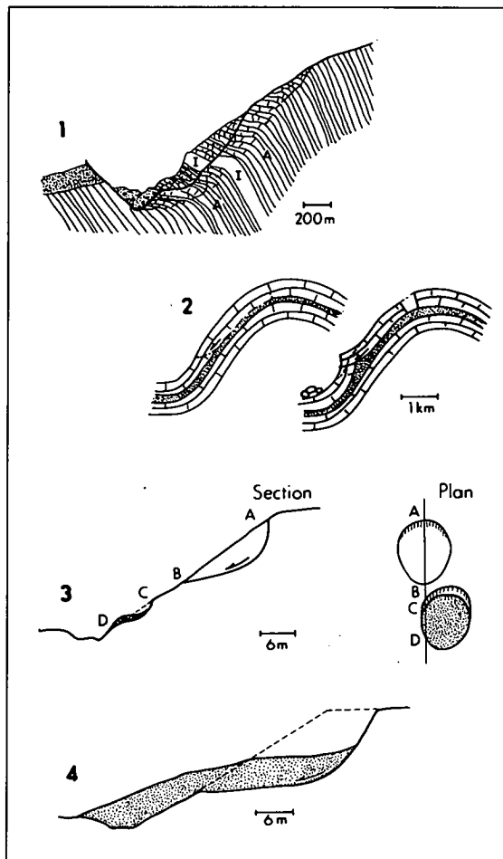
FIGURE 3-13 Sections through landslides showing different styles of activity. (1) Complex : gneiss (A) and migmatites (I) are forming topples caused by valley incision; alluvial materials fill valley bottom; after weathering further weakens toppled material, some of displaced mass moves by sliding (modified from Giraud et al. 1990). (2) Composite : limestones have slid on underlying shales, causing toppling failures below toe of slide rupture surface (modified from Harrison and Falcon 1934). (3) Successive : later landslide (AB) is same type as landslide CD but does not share displaced material or rupture surface. (4) Single .
